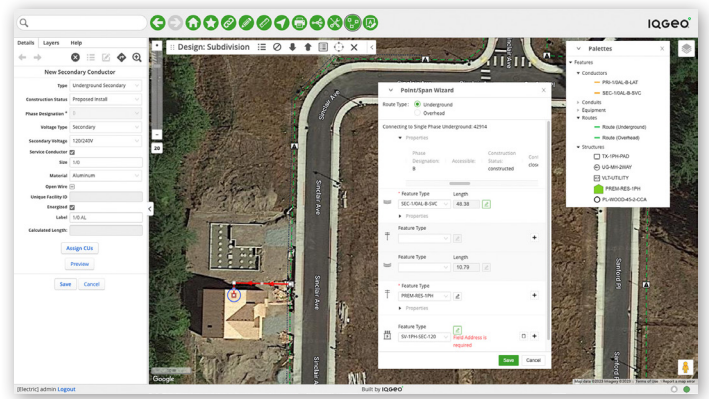
Easily add a new secondary conductor with the Point & Span wizard
